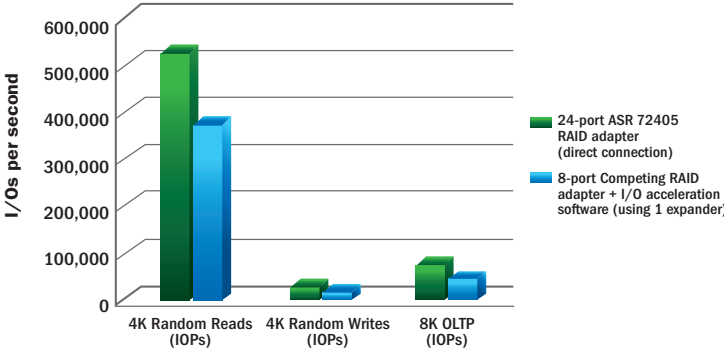
Figure 4. RAID 5 Performance (24 SAS SSDs)
