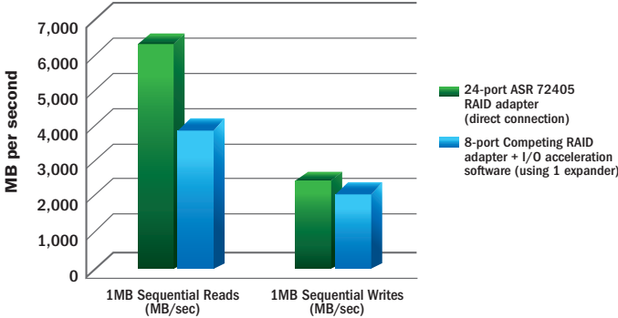
Figure 5. RAID 5 Sequential Performance (24 SAS SSDs)
